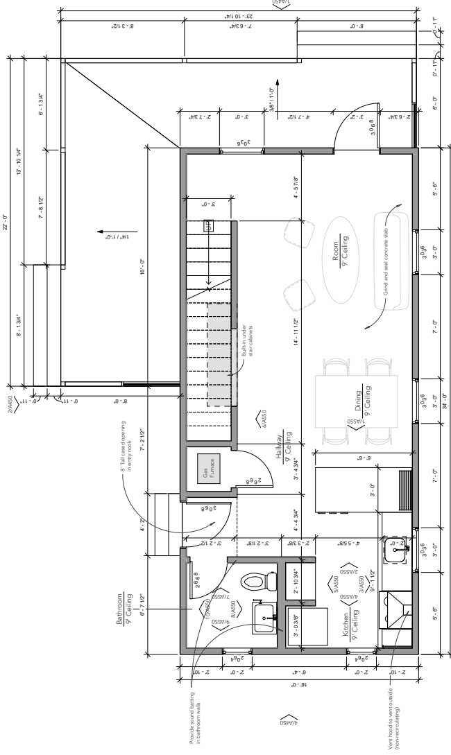
1 First Floor Plan 3/8" = 1'-0"
